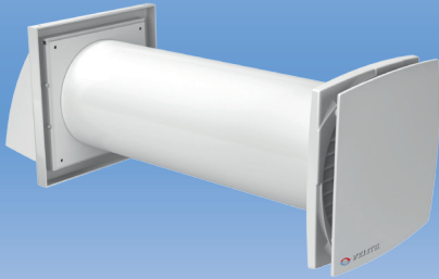
Wall ventilator with heat and energy recovery
