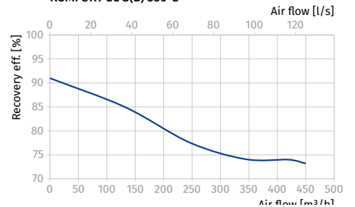
KOMFORT EC S(B) 350-E
